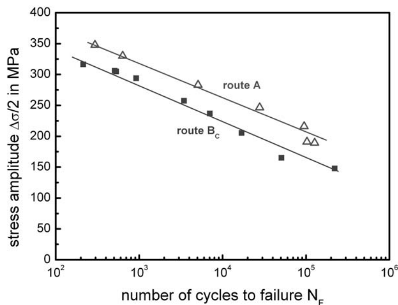
Figure 1. Wöhler (S-N) plot of UFG AlMg1.5 after 8 ECAP passes with ECAP route A and B c
