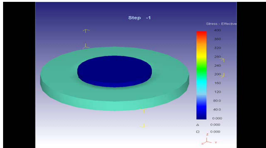
Figure 2. High pressure torsion simulation
