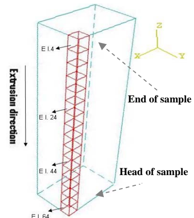
Figure 3. Partial discretized sample model with elemental corner path in red and elements specified numbered 4, 24, 44 and 64.
