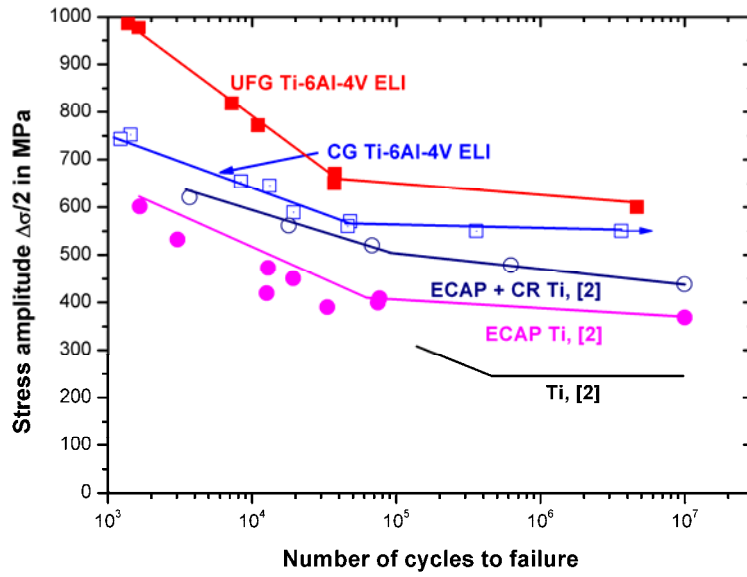
Figure 1. Wöhler S-N Diagrams of UFG and CG Ti-6Al-4V ELI alloy
