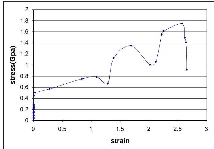
Figure 4. Diagram of Stress versus strain for 3 pass of TE of Ti-6Al-4V in element No. 4
