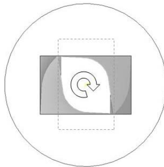
Figure 2. Schematic of 90° clockwise twist die (upside view). The exit outlet is shown in dashed line.
