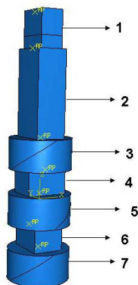
Figure 1. Schematic of TE setup for 2 passes. 1) Ram, 2) first guide, 3) first die, 4) second guide, 5) second die, 6) third guide and 7) third die.
