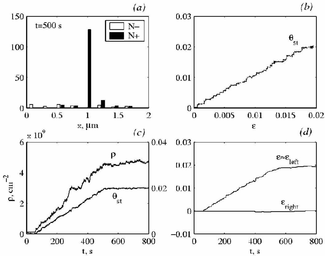
Figure 1. Distribution of number of dislocations, characteristics of sub-boundary and values of strain at the both sides of the boundary: (a) – histogram of number of dislocations with different sign ( N_+ and N_- ) at t = 500 s; (b) – the dependence of sub-boundary misorientation \theta_{st} on the value of strain \epsilon = \epsilon_{left} + \epsilon_{right} ; (c) – time dependences of the average dislocations density in the body of grain \rho and sub-boundary misorientation \theta_{st} ; (d) – the time dependence of the value of strain to the left \epsilon_{left} and right \epsilon_{right} sides of sub-boundary
