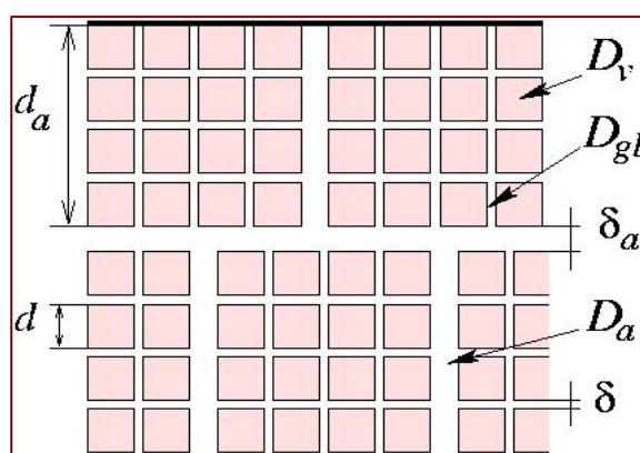
Figure 1. Schematic presentation of hierarchical microstructure of the bulk nanocrystalline Fe-Ni alloy
