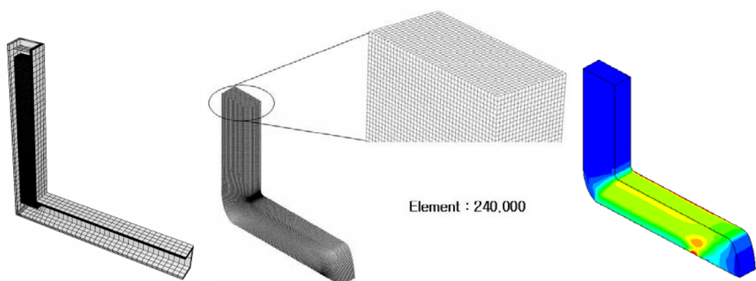
Figure 1. Mesh system of 3-dimensional: initial mesh, deformed mesh and strain distribution
