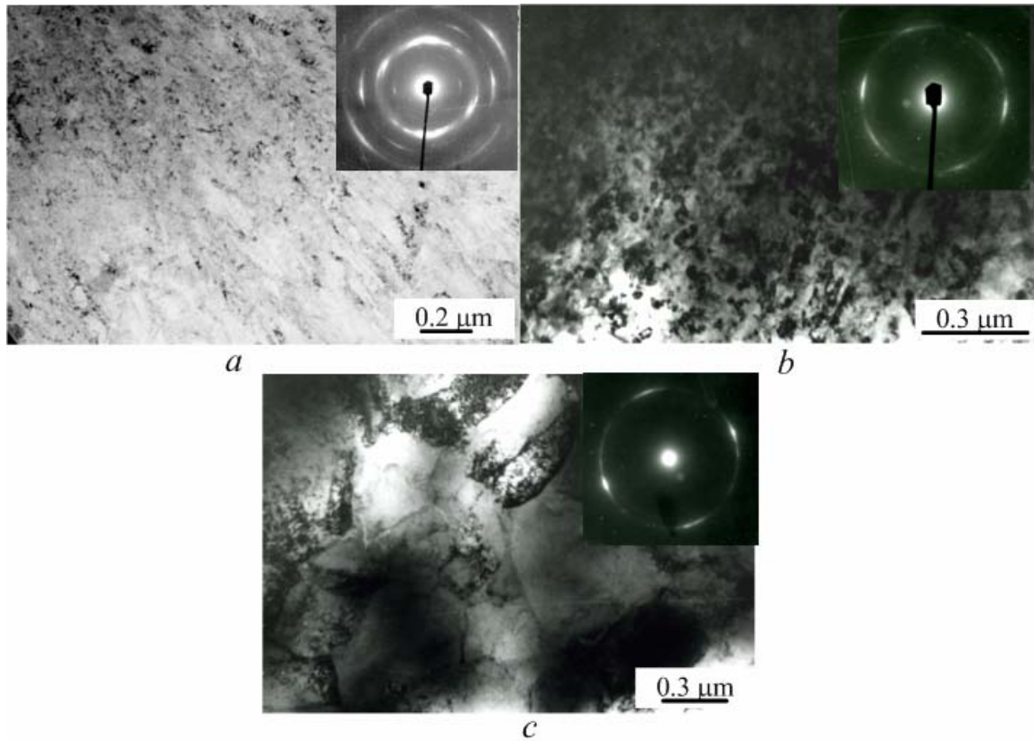
Figure 1. Structures and electron diffraction patterns of Ti-50.7 %Ni alloy directly after EPD, e=0.8 under controlled current density (a), after subsequent post-deformation annealing at 400 \text{ }^\circ\text{C} (b), and directly after EPD, e=1.8 under constant current value (c)
